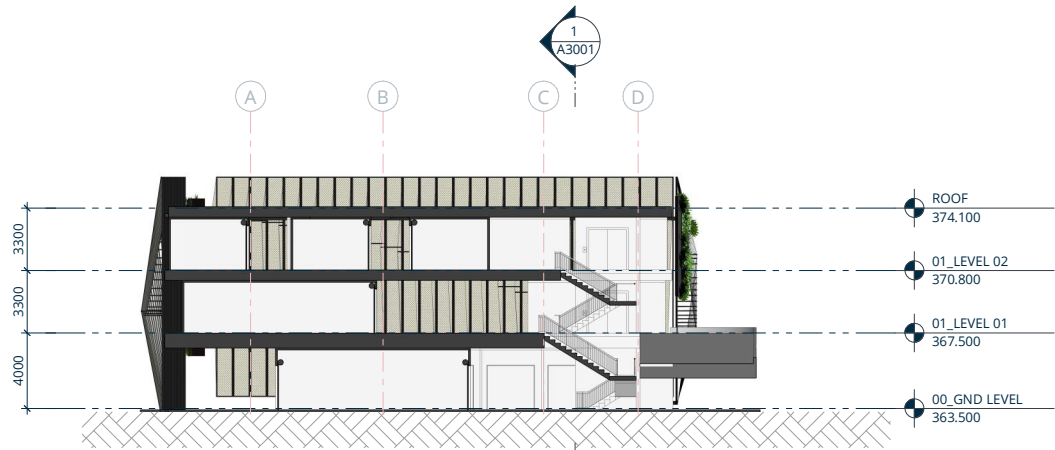
2 CROSS SECTION B A1301 SCALE @ A1: 1 : 200
