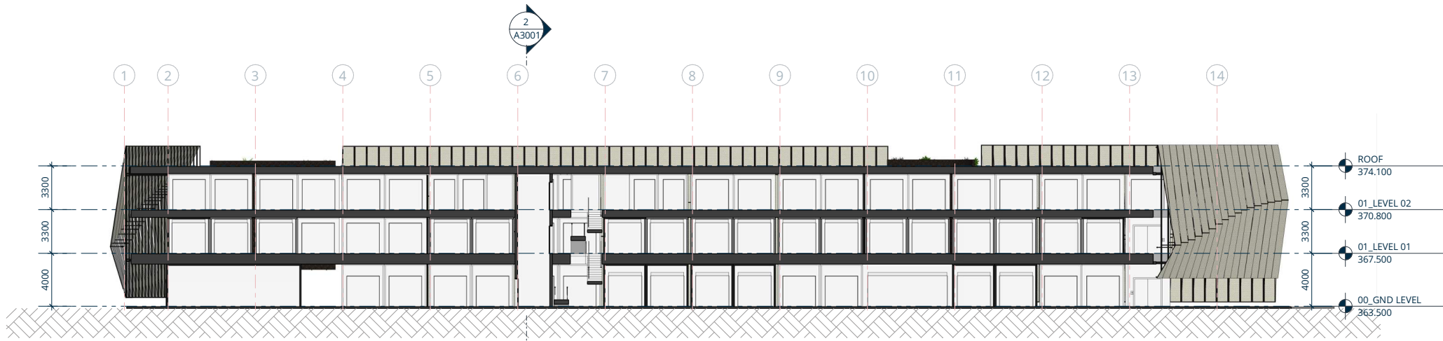
1 CROSS SECTION A A1301 SCALE @ A1: 1 : 200
