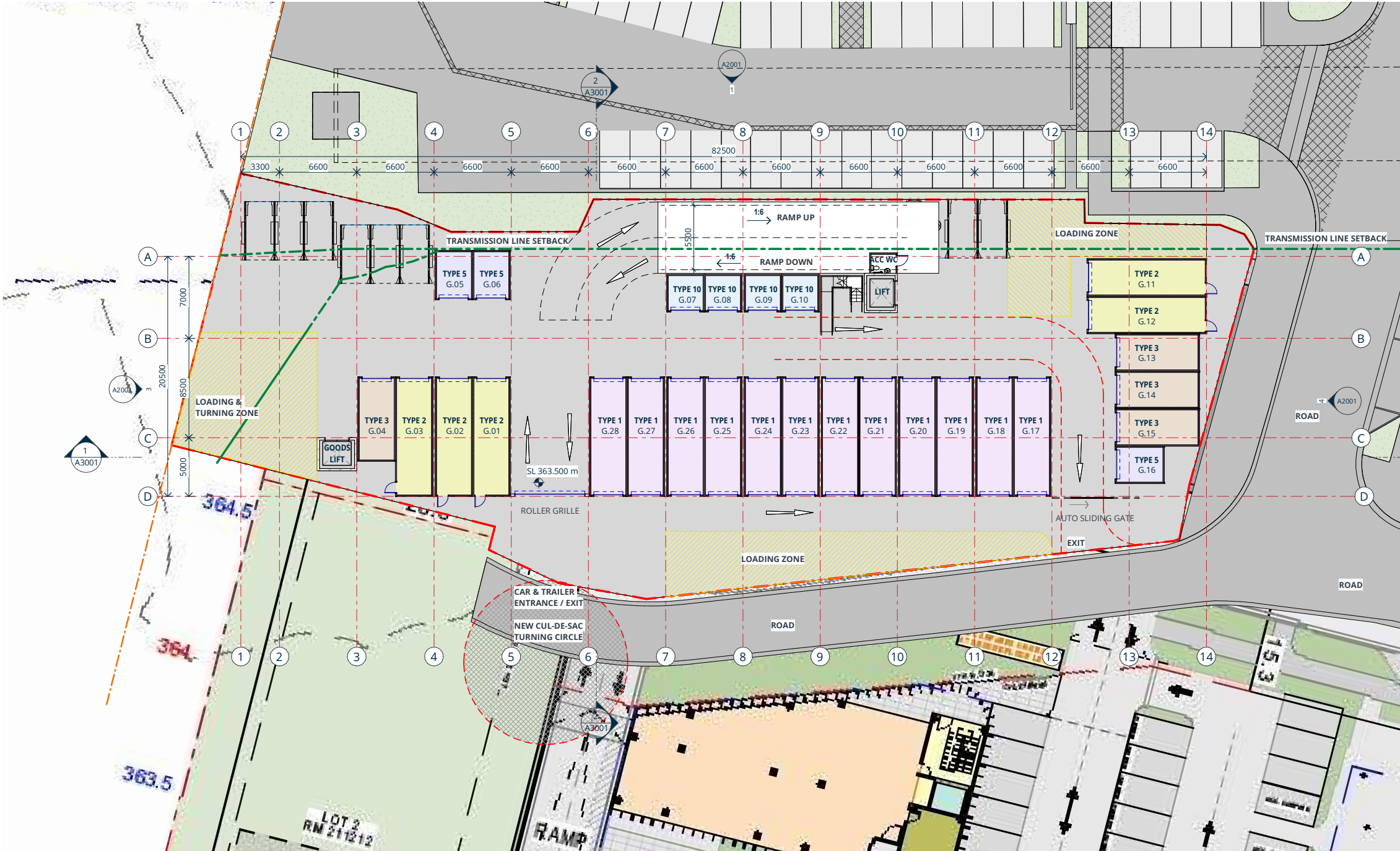
1 LEVEL 00 - GROUND FLOOR PLAN A2001 SCALE @ A1: 1 : 200
